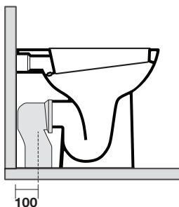
curva tecnica art. 900102 waste pipe art. 900102
